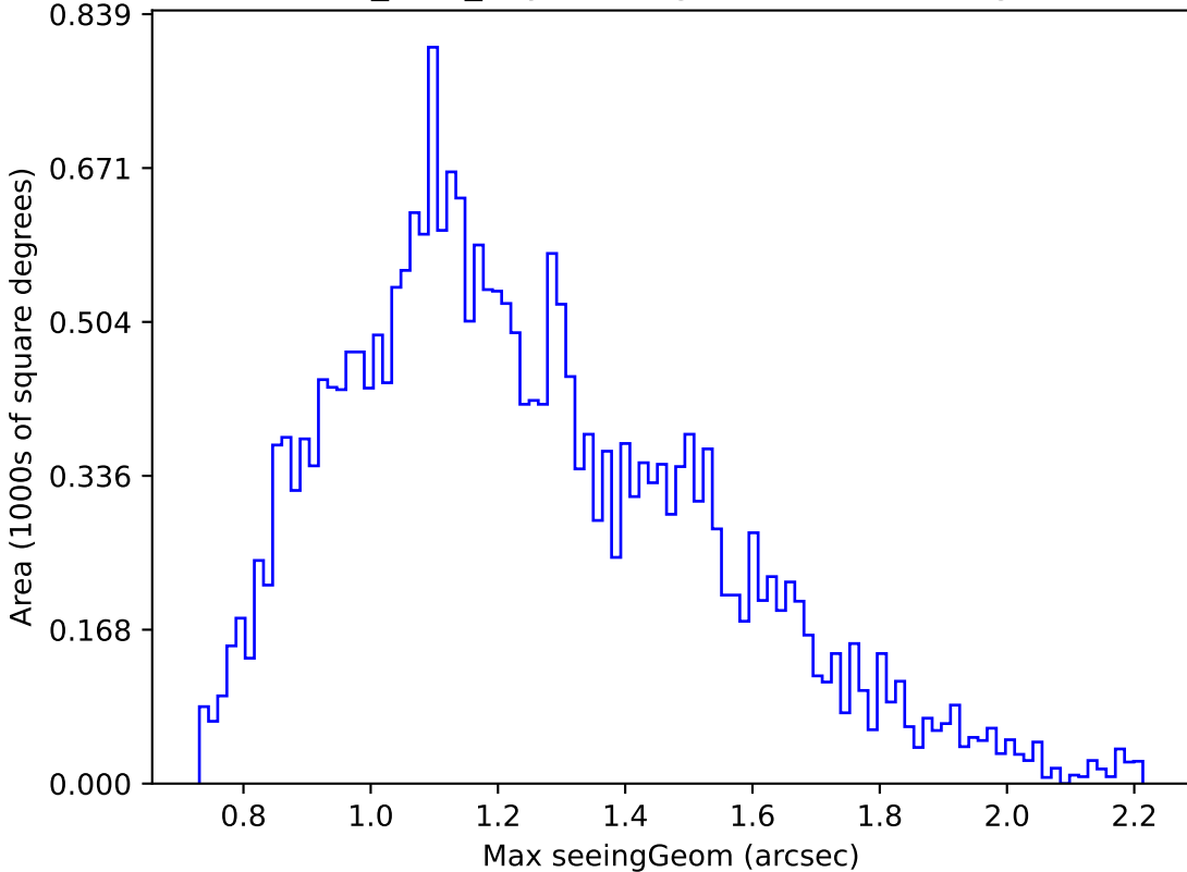
baseline_v3.0_10yrs Yr 1 g band: Max seeingGeom
