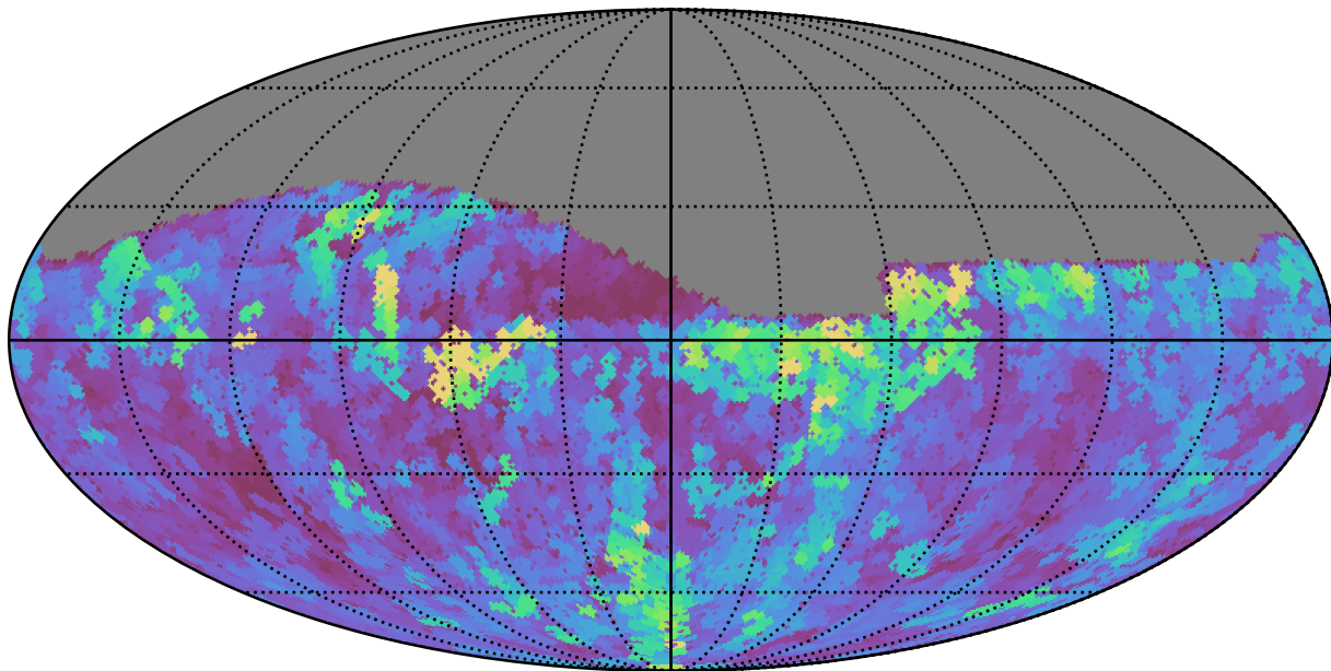
baseline_v3.0_10yrs Yr 1 all bands: Max seeingGeom
