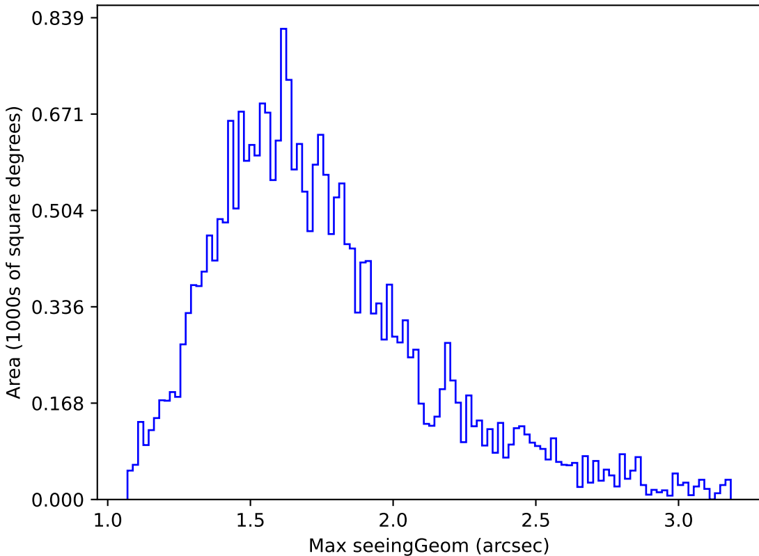
baseline_v3.0_10yrs Yr 1 all bands: Max seeingGeom
