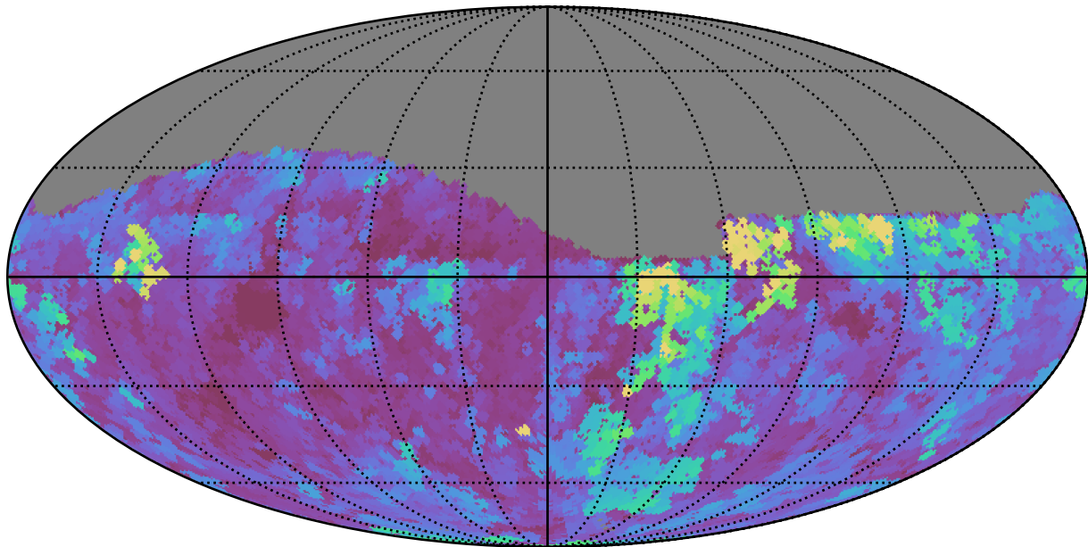
baseline_v3.0_10yrs Yr 1 z band: Max seeingEff
