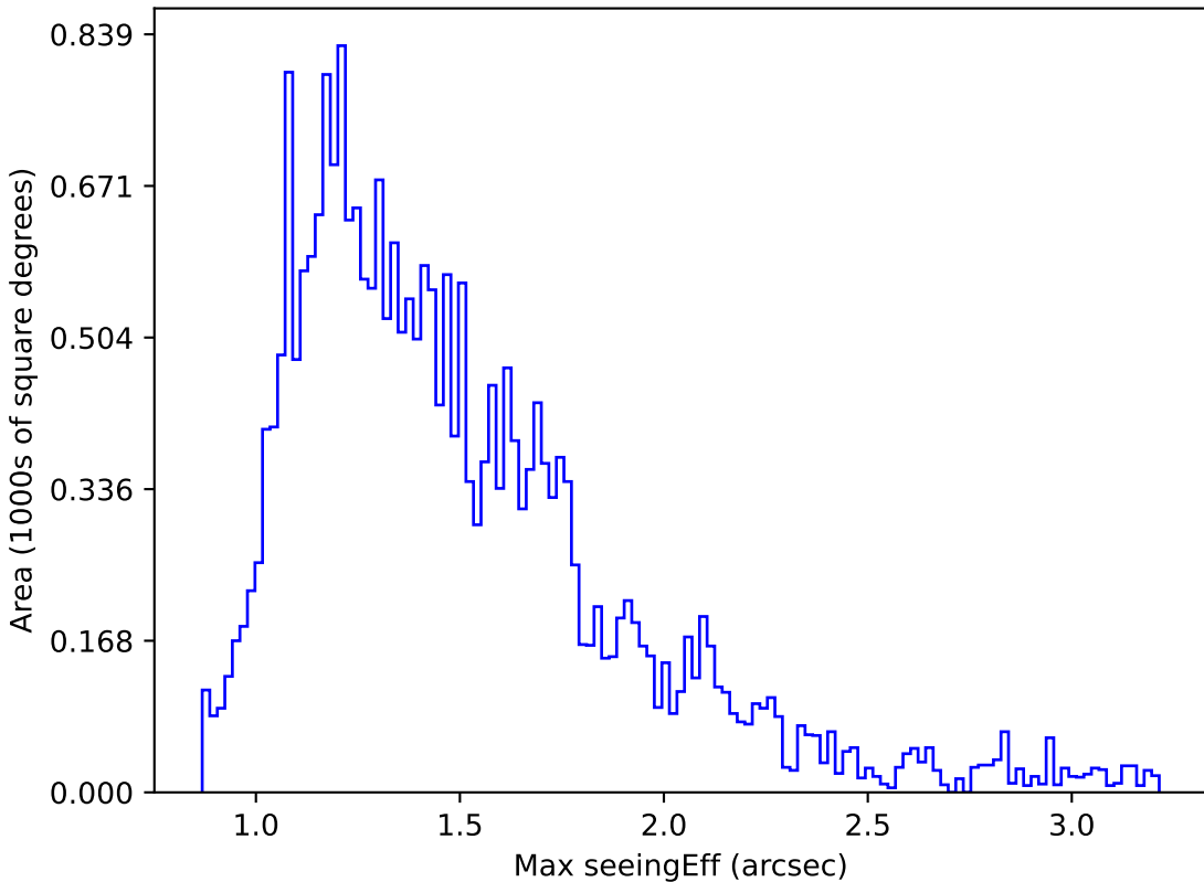
baseline_v3.0_10yrs Yr 1 z band: Max seeingEff
