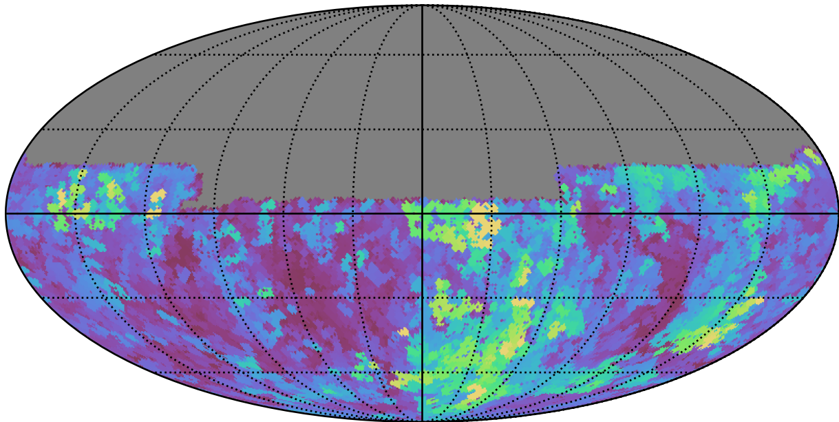
baseline_v3.0_10yrs Yr 1 y band: Max seeingEff
