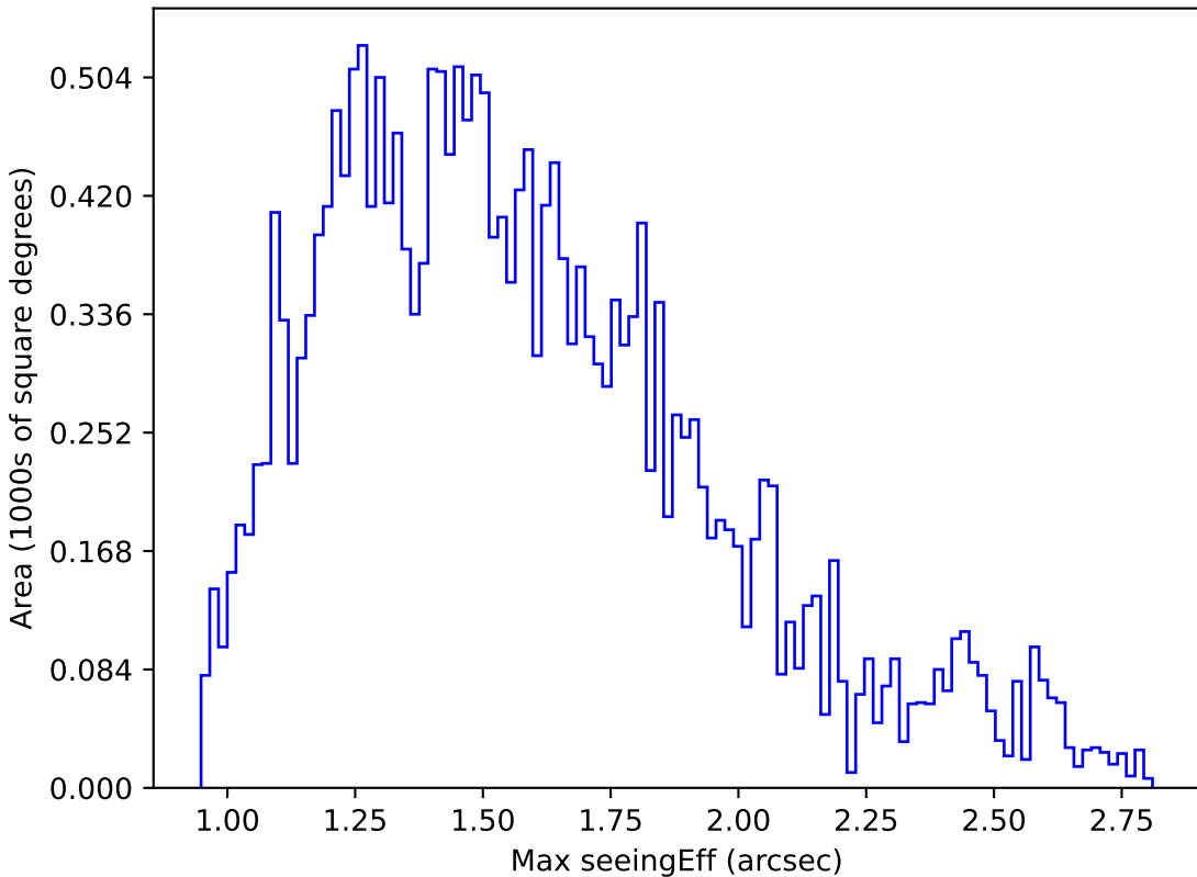
baseline_v3.0_10yrs Yr 1 y band: Max seeingEff
