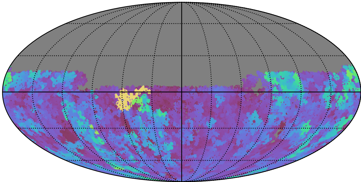
baseline_v3.0_10yrs Yr 1 u band: Max seeingEff
