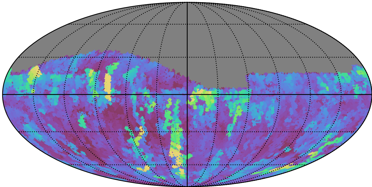
baseline_v3.0_10yrs Yr 1 r band: Max seeingEff
