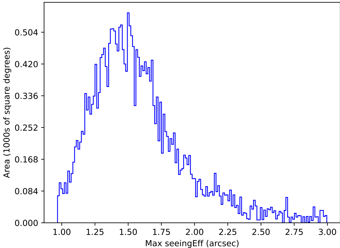
baseline_v3.0_10yrs Yr 1 r band: Max seeingEff
