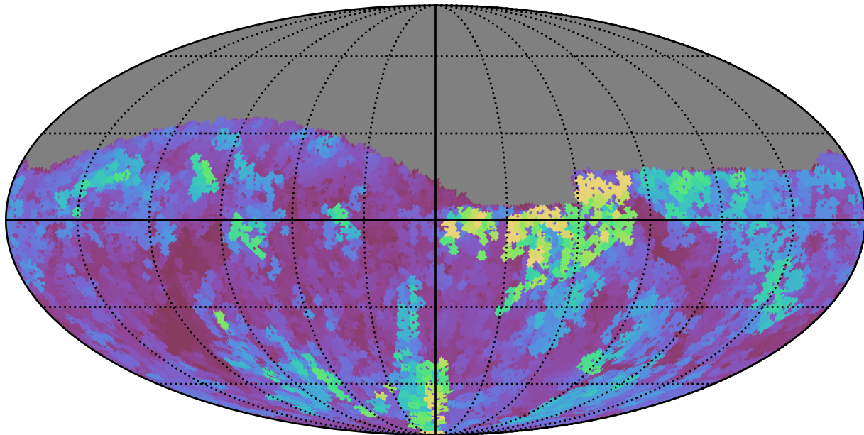
baseline_v3.0_10yrs Yr 1 i band: Max seeingEff
