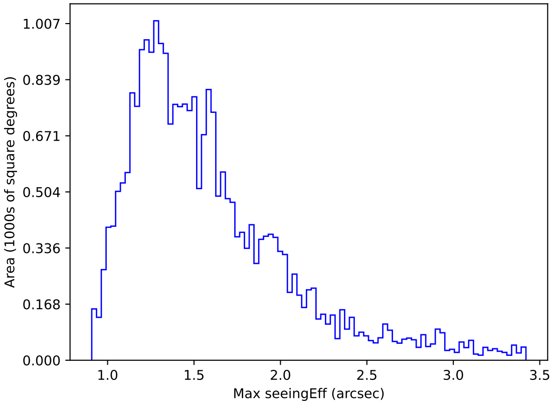
baseline_v3.0_10yrs Yr 1 i band: Max seeingEff
