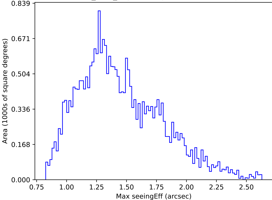
baseline_v3.0_10yrs Yr 1 g band: Max seeingEff
