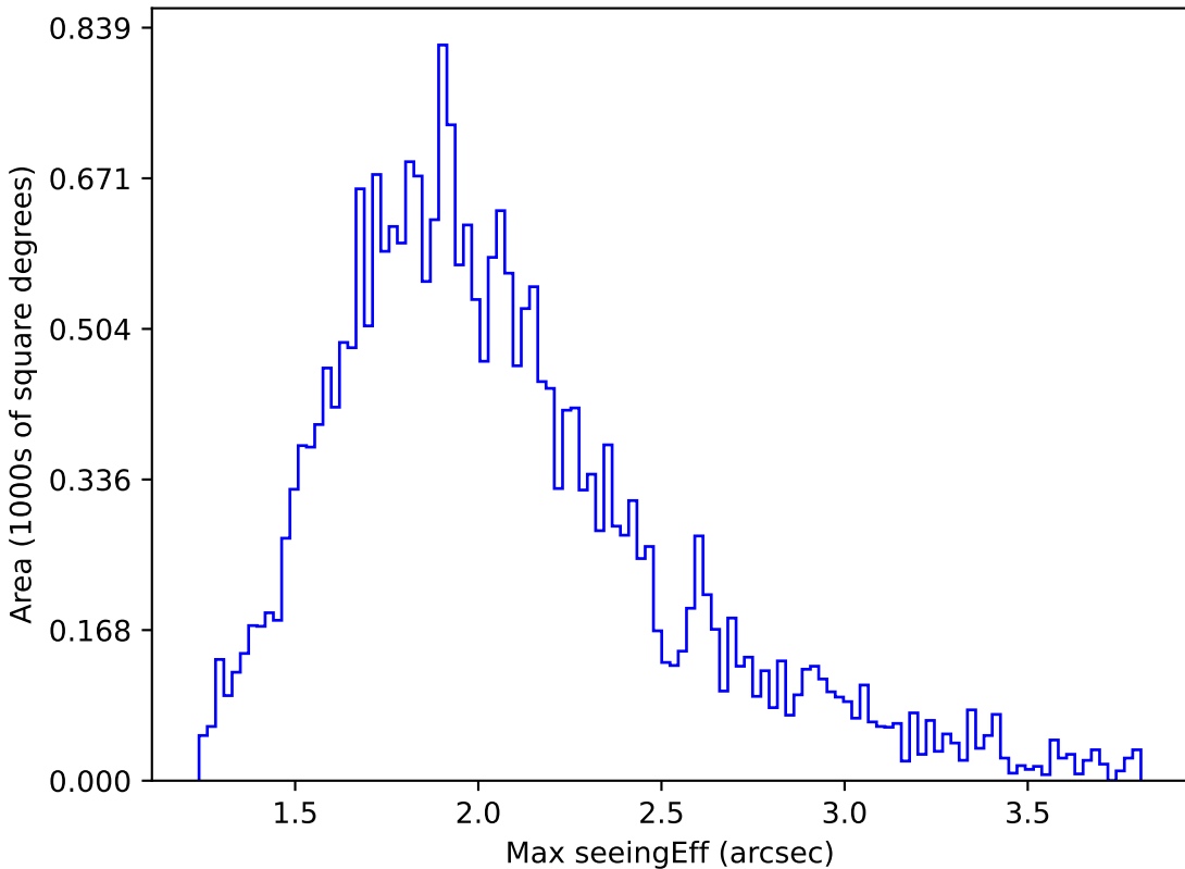
baseline_v3.0_10yrs Yr 1 all bands: Max seeingEff
