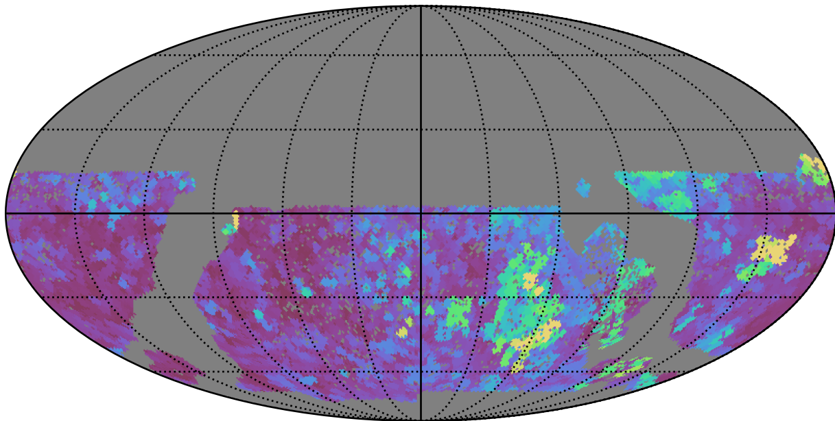
baseline_v3.0_10yrs WFD z band: Max seeingEff
