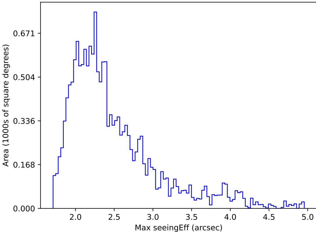
baseline_v3.0_10yrs WFD z band: Max seeingEff
