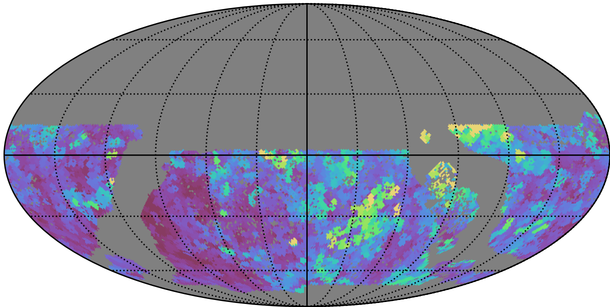
baseline_v3.0_10yrs WFD y band: Max seeingEff
