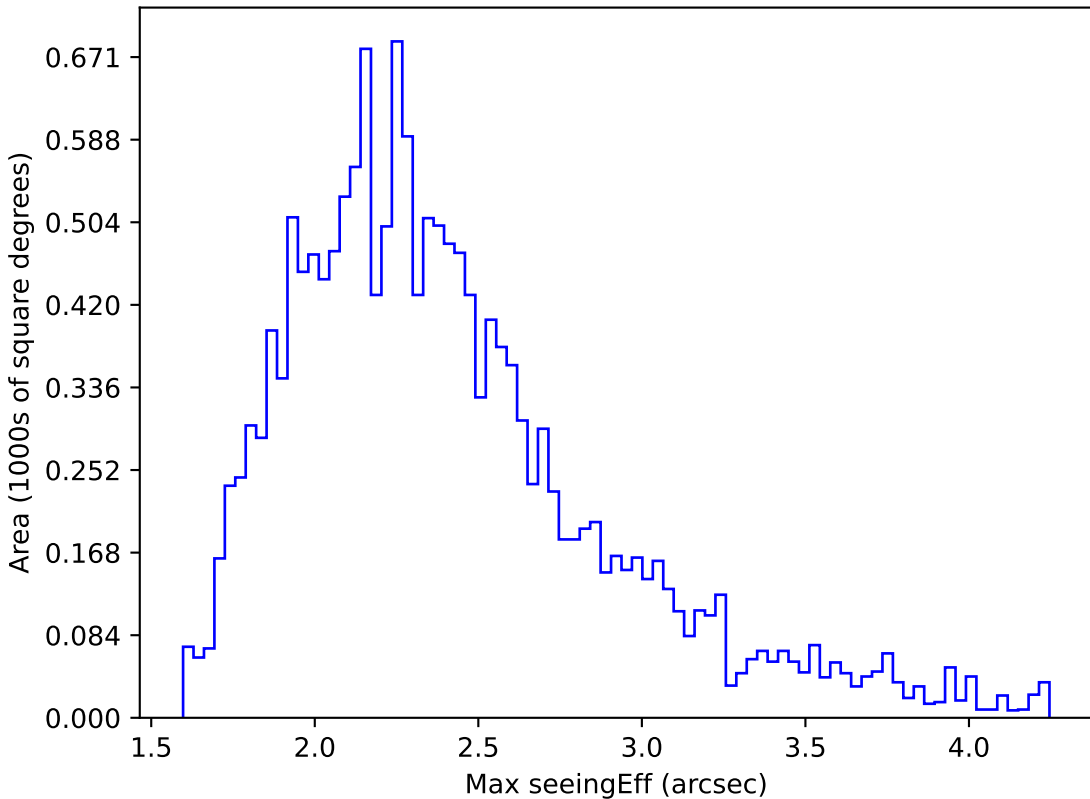
baseline_v3.0_10yrs WFD y band: Max seeingEff
