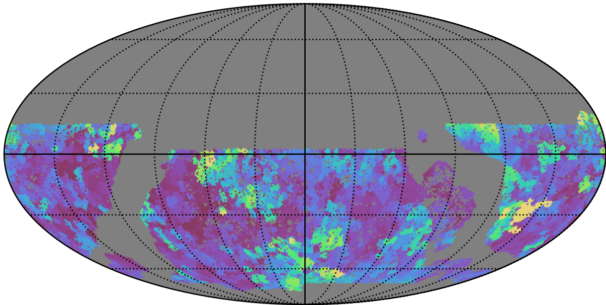
baseline_v3.0_10yrs WFD u band: Max seeingEff
