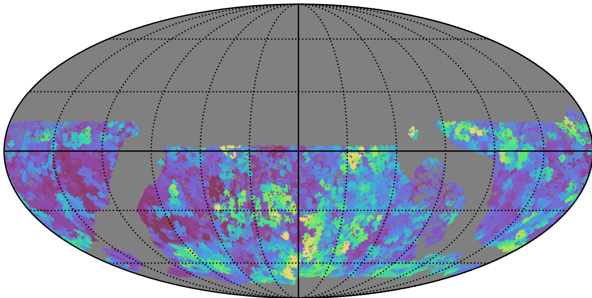
baseline_v3.0_10yrs WFD r band: Max seeingEff
