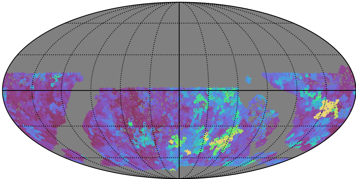
baseline_v3.0_10yrs WFD i band: Max seeingEff
