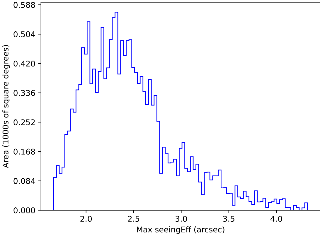
baseline_v3.0_10yrs WFD g band: Max seeingEff
