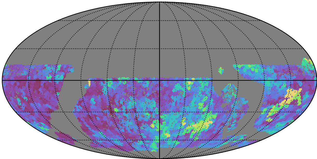
baseline_v3.0_10yrs WFD all bands: Max seeingEff
