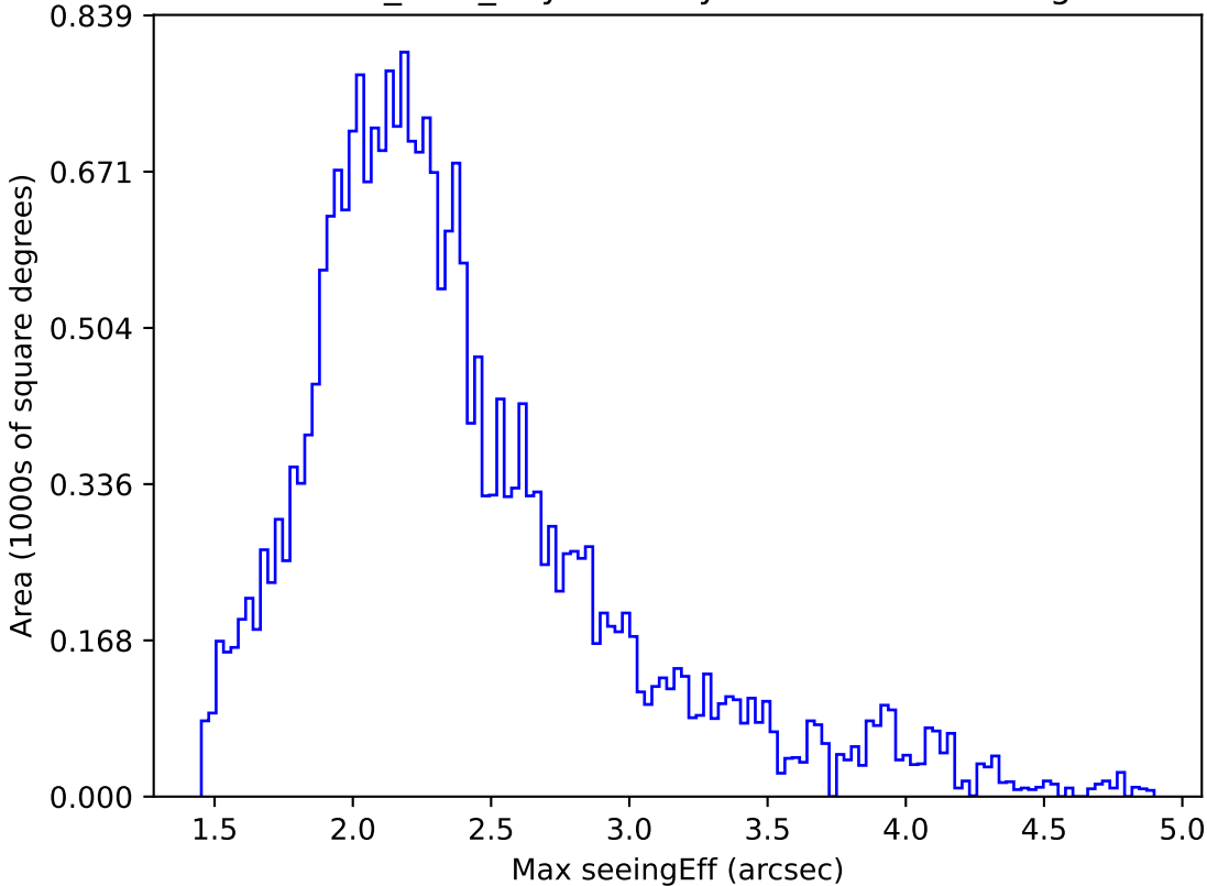
baseline_v3.0_10yrs All sky z band: Max seeingEff
