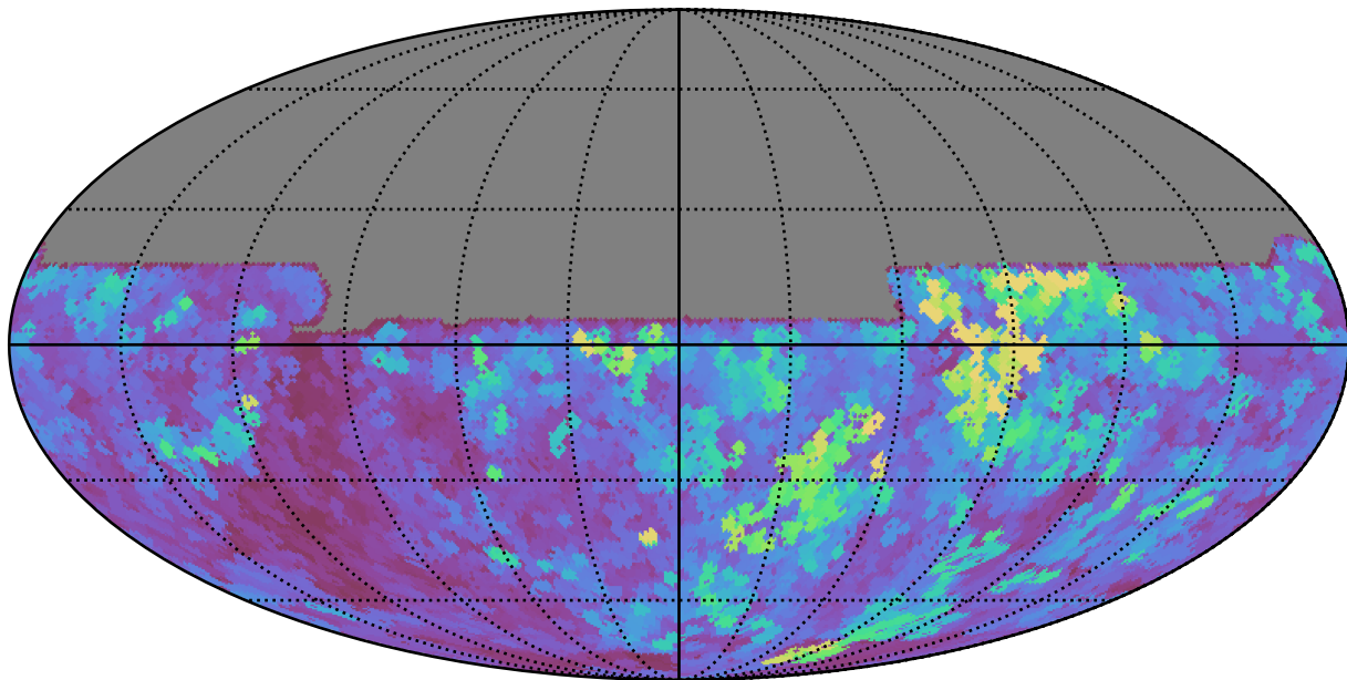
baseline_v3.0_10yrs All sky y band: Max seeingEff
