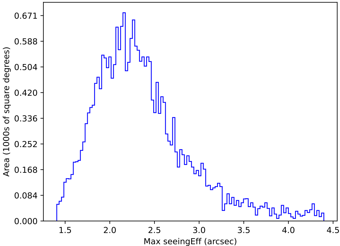
baseline_v3.0_10yrs All sky y band: Max seeingEff
