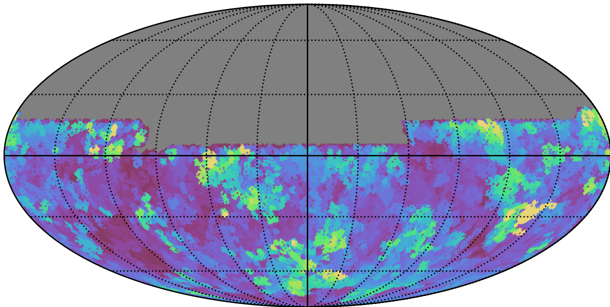
baseline_v3.0_10yrs All sky u band: Max seeingEff
