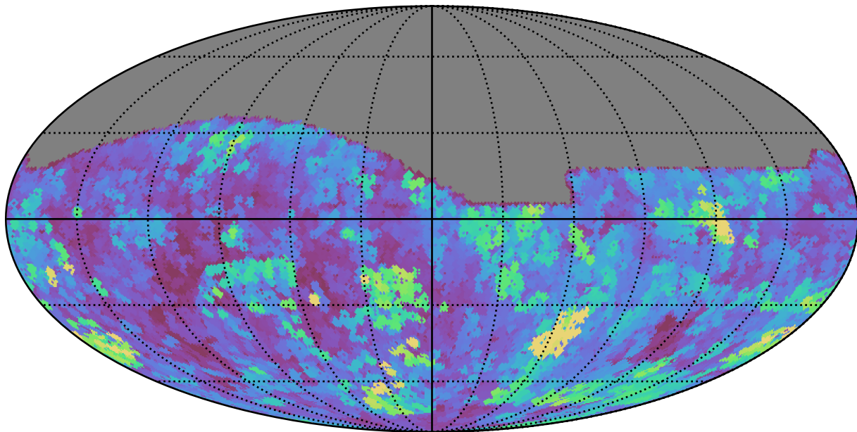
baseline_v3.0_10yrs All sky g band: Max seeingEff
