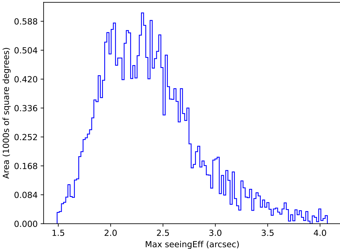
baseline_v3.0_10yrs All sky g band: Max seeingEff
