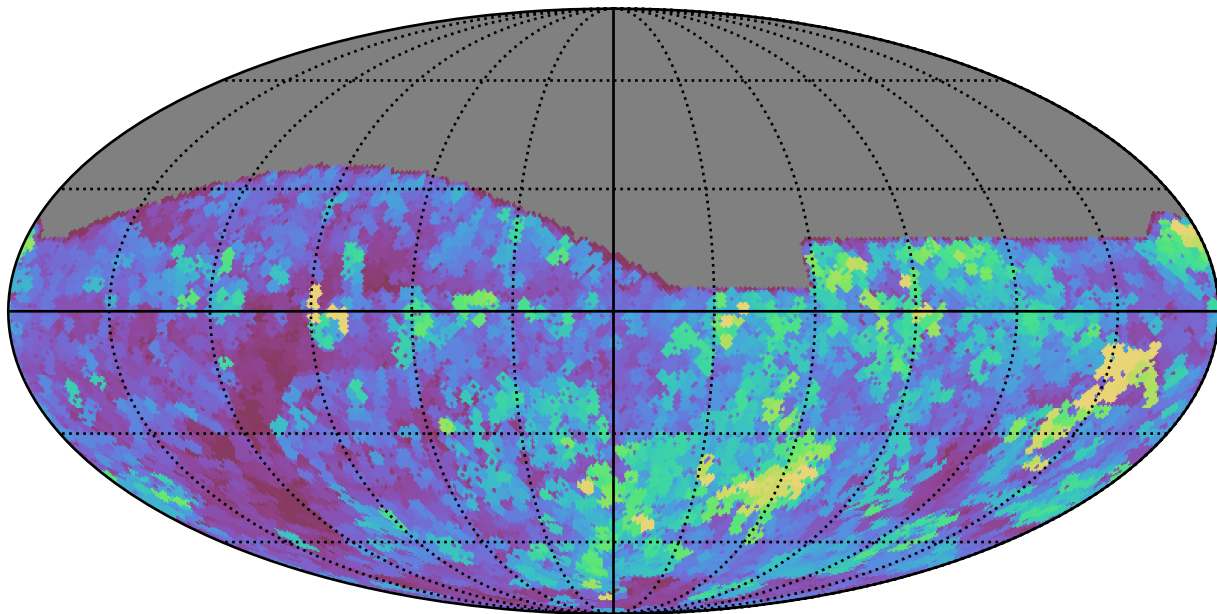
baseline_v3.0_10yrs All sky all bands: Max seeingEff
