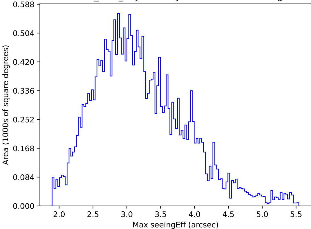
baseline_v3.0_10yrs All sky all bands: Max seeingEff
