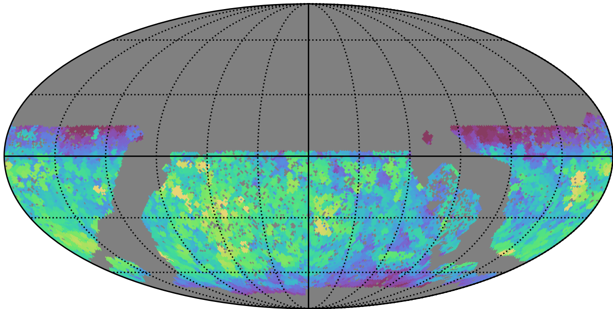
baseline_v3.0_10yrs WFD z band: Max saturation_mag
