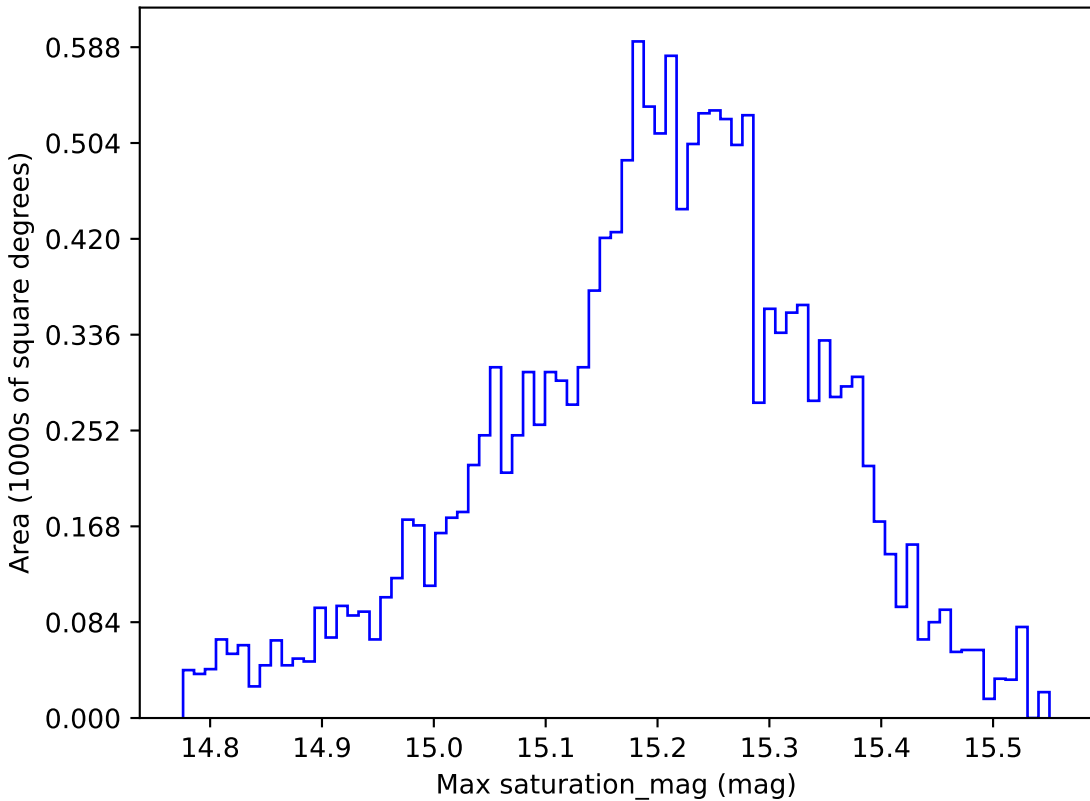
baseline_v3.0_10yrs WFD z band: Max saturation_mag
