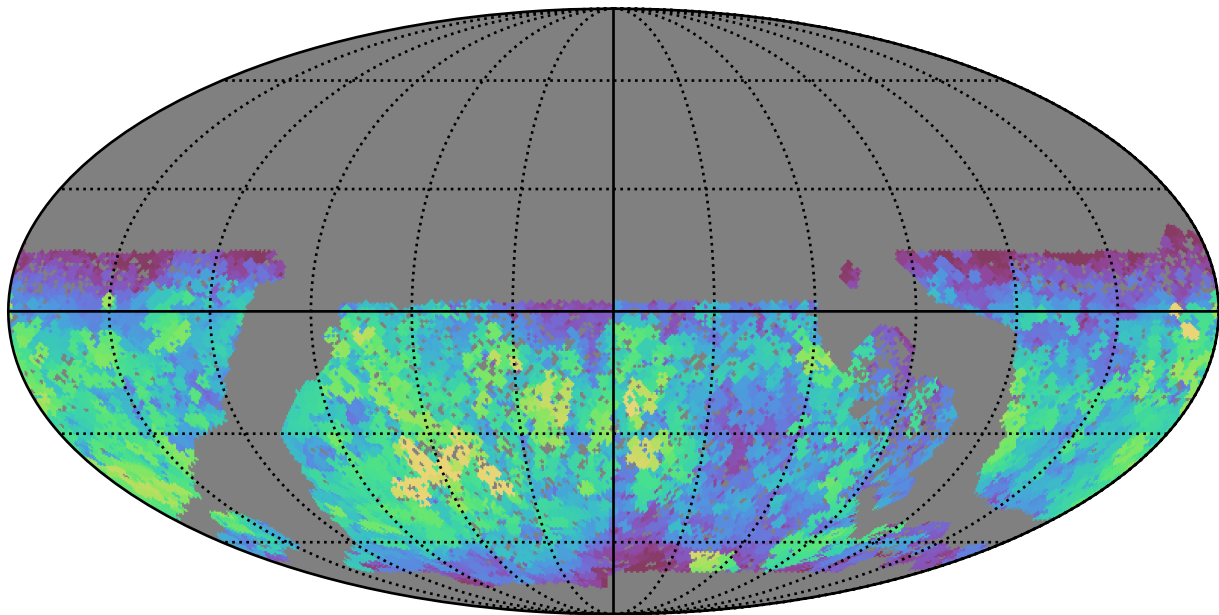
baseline_v3.0_10yrs WFD y band: Max saturation_mag
