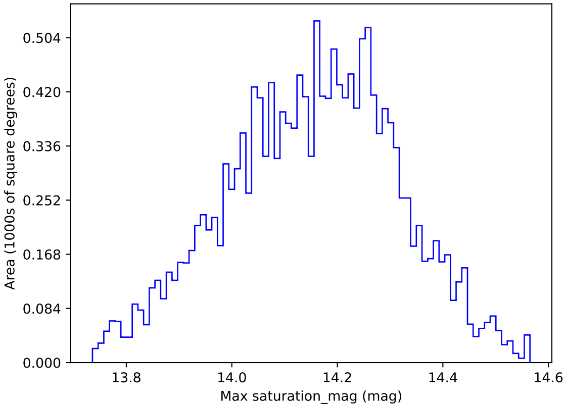
baseline_v3.0_10yrs WFD y band: Max saturation_mag
