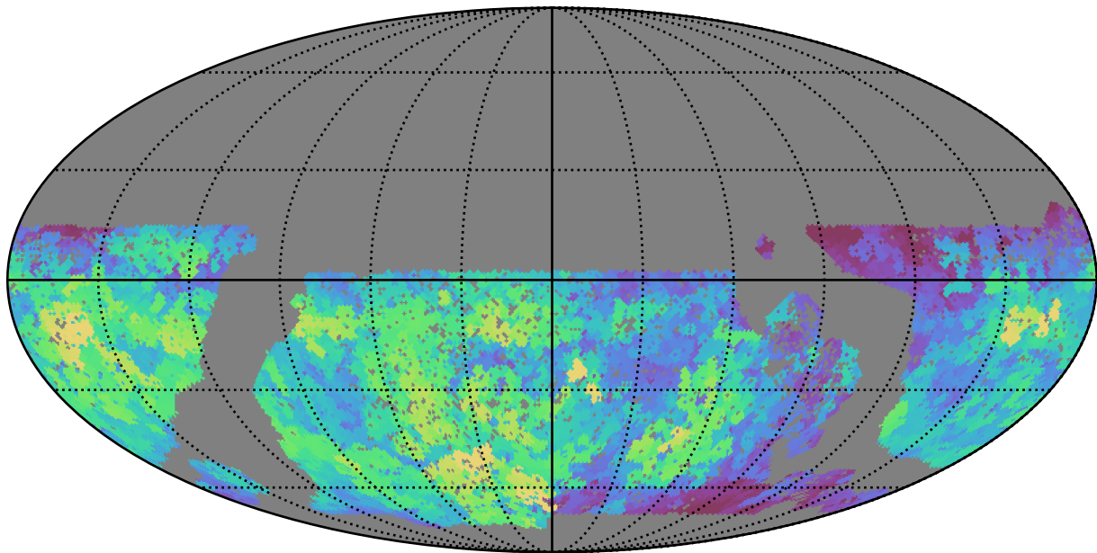
baseline_v3.0_10yrs WFD u band: Max saturation_mag
