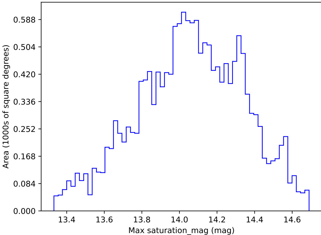
baseline_v3.0_10yrs WFD u band: Max saturation_mag
