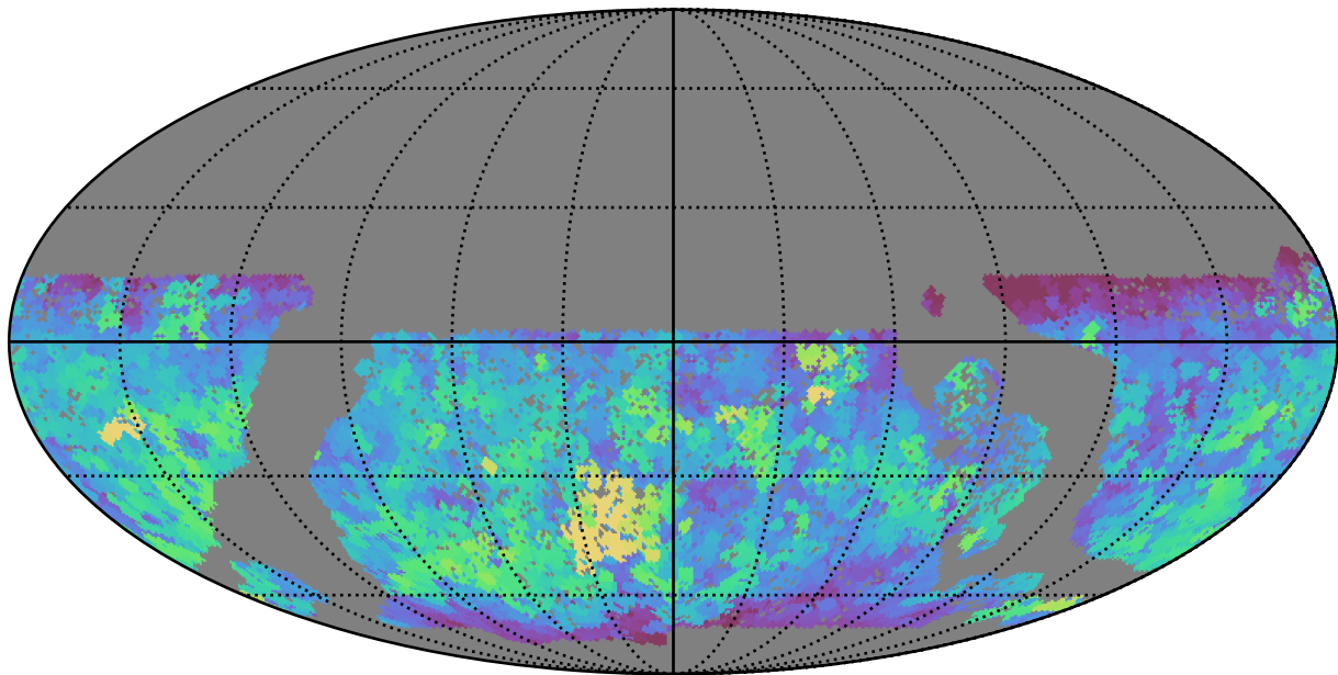
baseline_v3.0_10yrs WFD r band: Max saturation_mag
