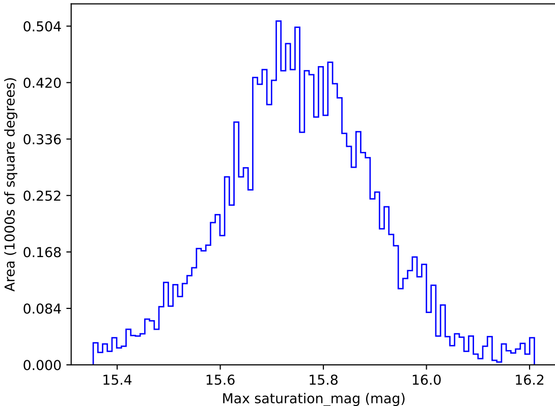
baseline_v3.0_10yrs WFD r band: Max saturation_mag
