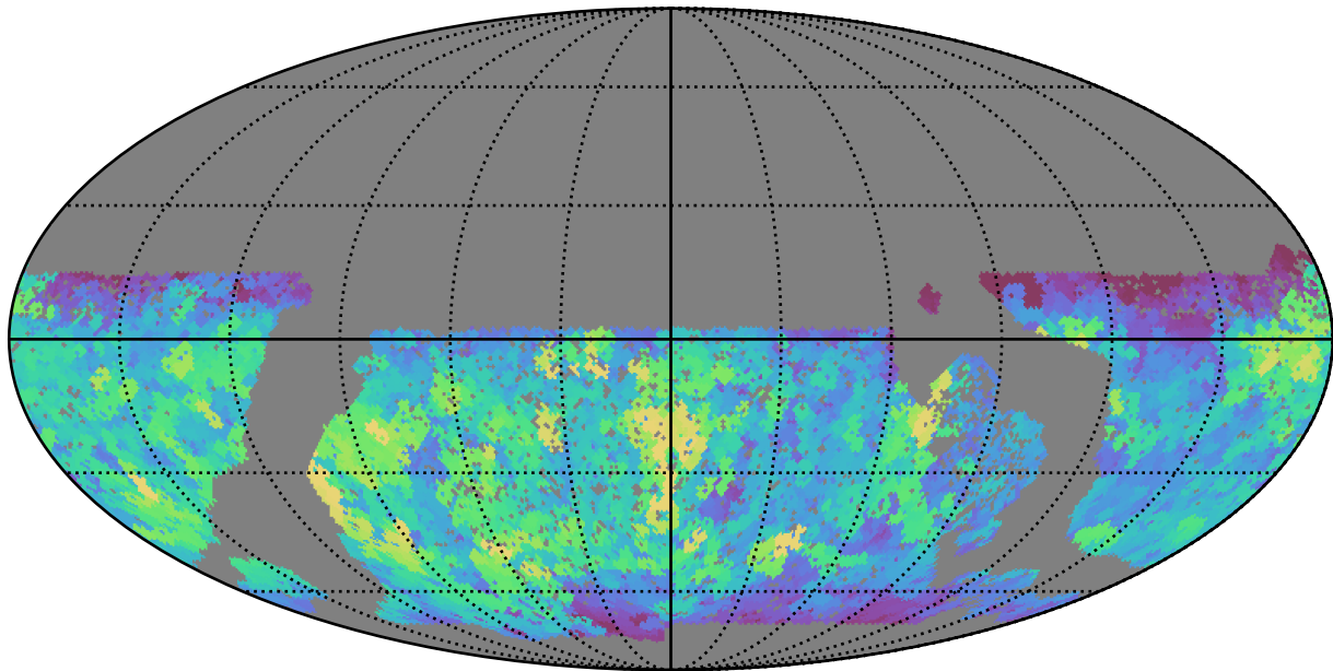
baseline_v3.0_10yrs WFD i band: Max saturation_mag
