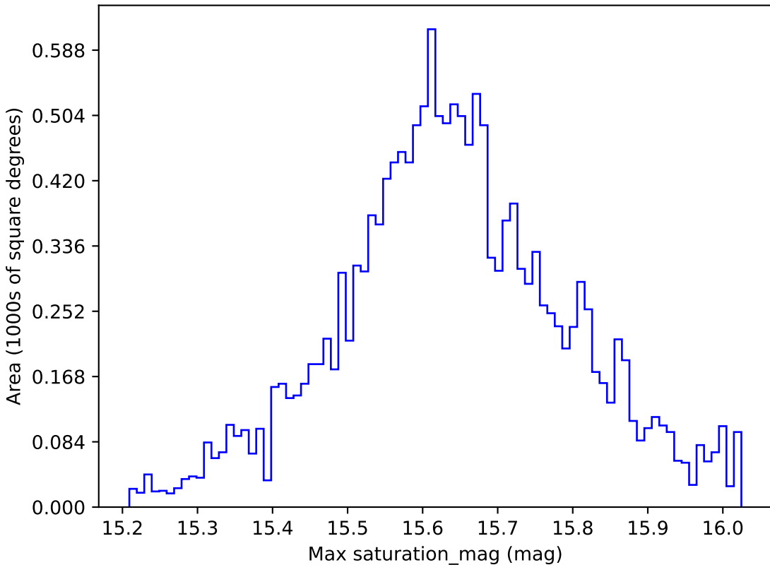
baseline_v3.0_10yrs WFD i band: Max saturation_mag
