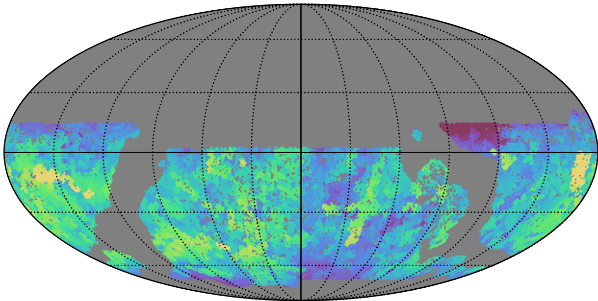
baseline_v3.0_10yrs WFD g band: Max saturation_mag
