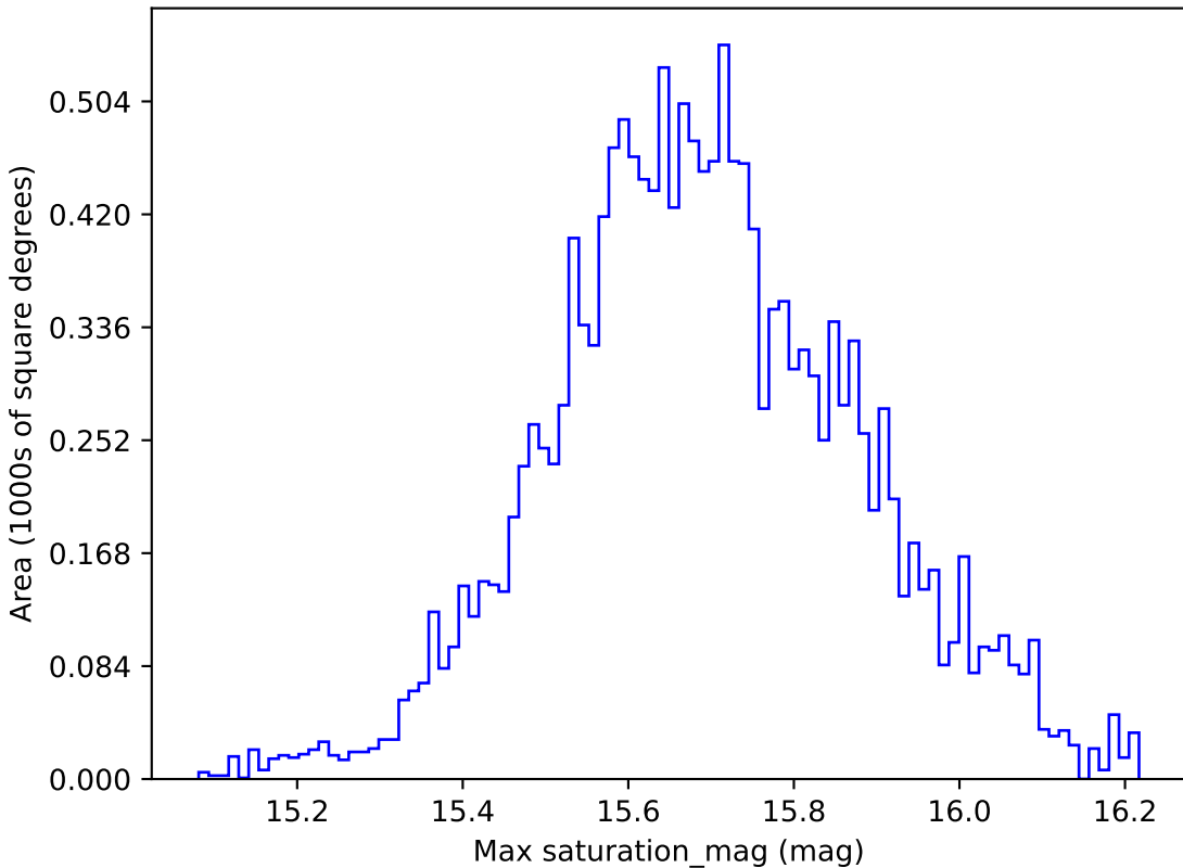
baseline_v3.0_10yrs WFD g band: Max saturation_mag
