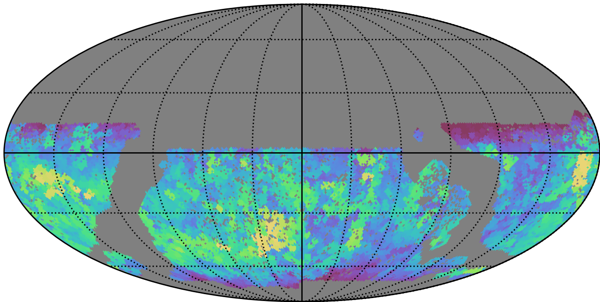
baseline_v3.0_10yrs WFD all bands: Max saturation_mag
