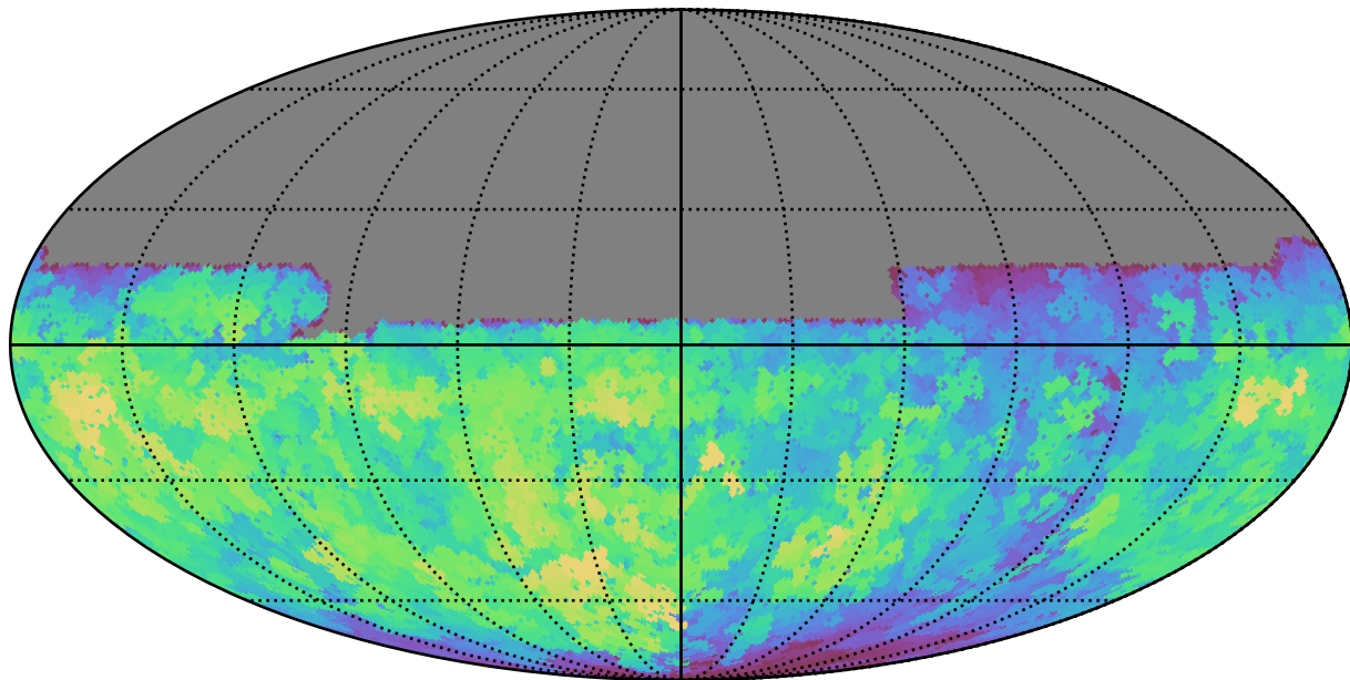
baseline_v3.0_10yrs All sky u band: Max saturation_mag
