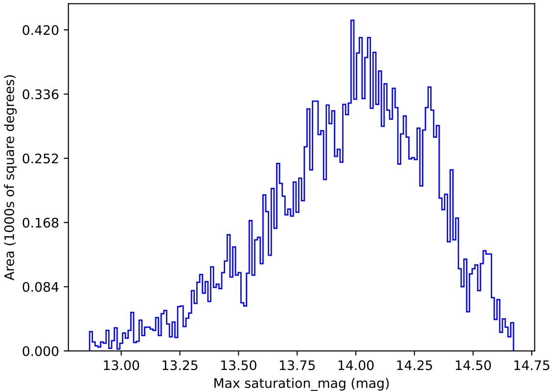
baseline_v3.0_10yrs All sky u band: Max saturation_mag
