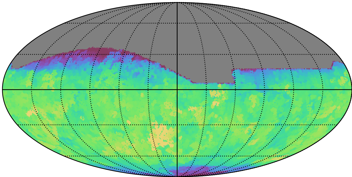
baseline_v3.0_10yrs All sky r band: Max saturation_mag
