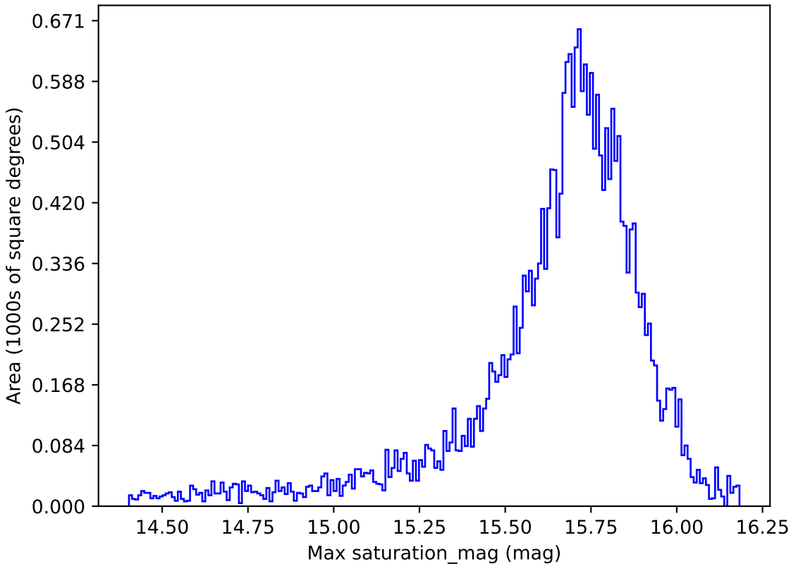
baseline_v3.0_10yrs All sky r band: Max saturation_mag
