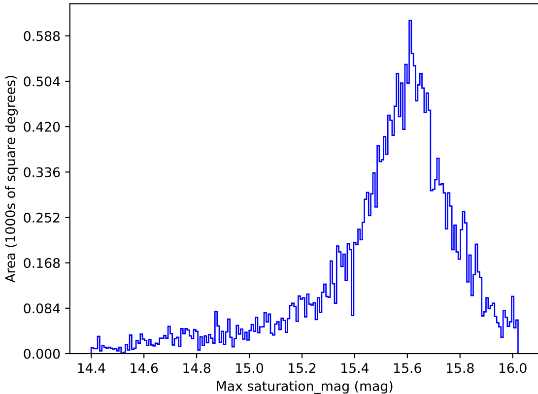
baseline_v3.0_10yrs All sky i band: Max saturation_mag
