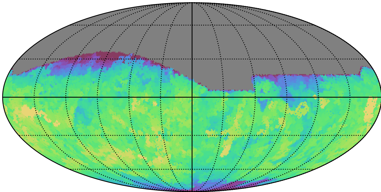
baseline_v3.0_10yrs All sky g band: Max saturation_mag
